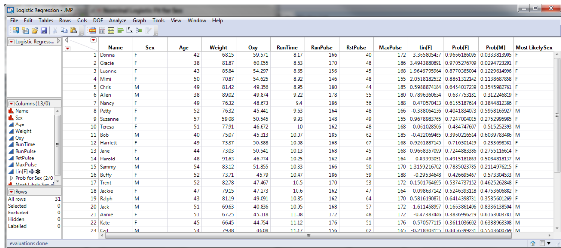
Fig. 4.63 Logistic Regression Predictions
