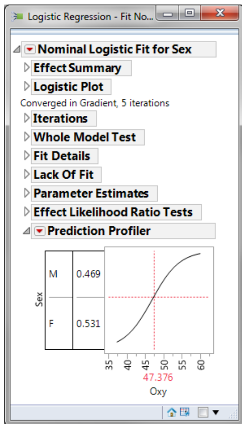
Fig. 4.64 Prediction Profiler output
