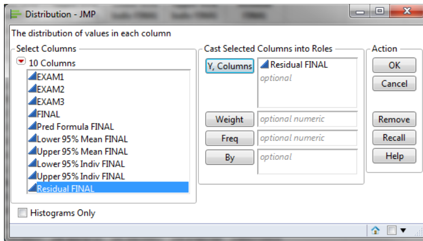
Fig. 4.35 Distribution selections
