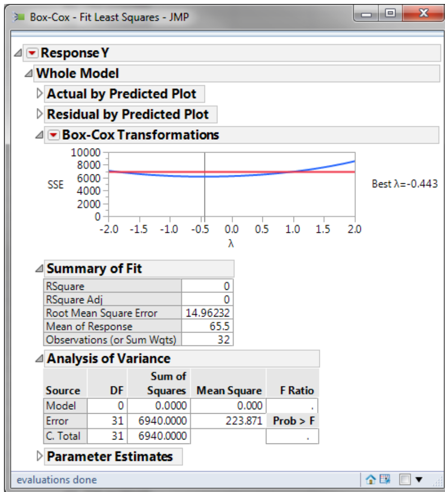
Fig. 4.44 Box-Cox Results
