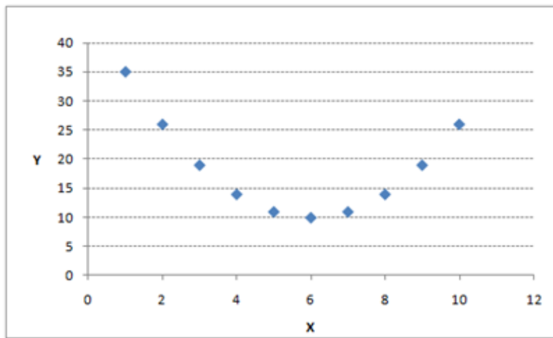
Fig. 4.7 Non-Linear Correlation
