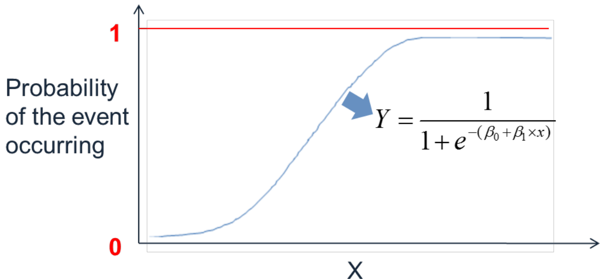
Fig. 4.52 Logistic Curve
