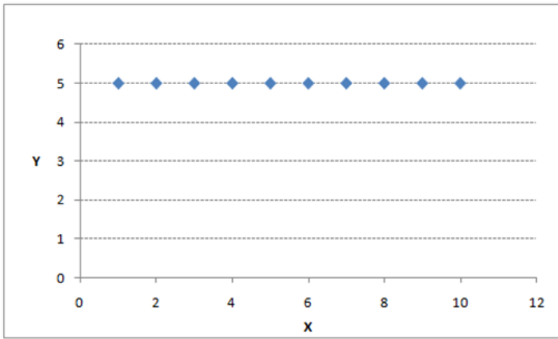
Fig. 4.8 Uncorrelated Correlation
