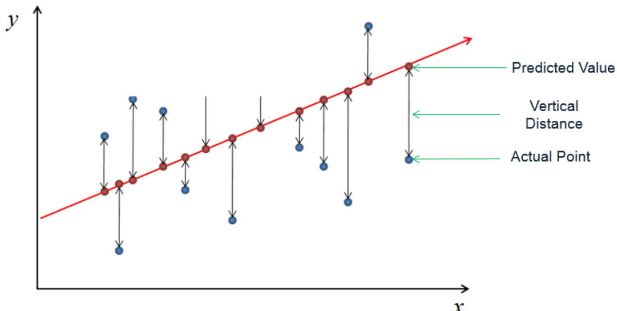
Fig. 4.17 Understanding Residuals
